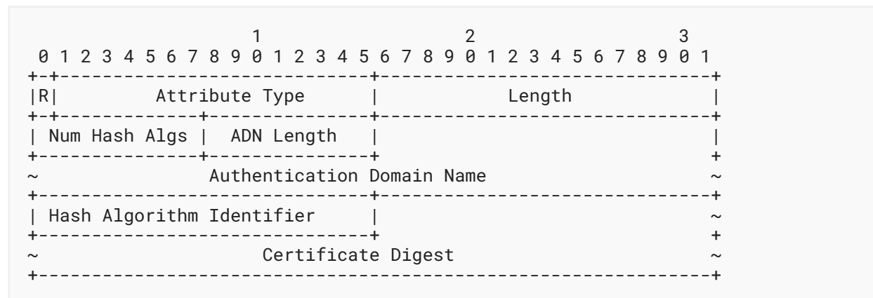
Figure 4: ENCDNS_DIGEST_INFO Attribute Format in CFG_REPLY or CFG_SET
